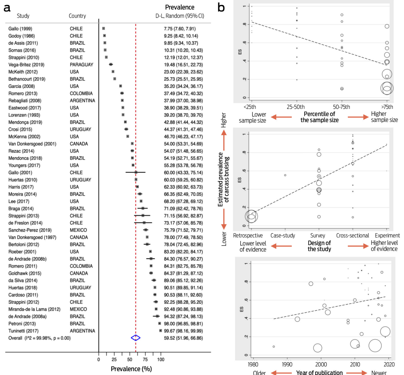
Figure 2. a) Forest plot of the 43 studies included in the meta-analysis for estimating the prevalence of carcass bruising in cattle from America, b) results of meta-regression analyses of the prevalence of carcass bruising according to the percentile of the sample size (upper panel), the design of the study (middle panel), and publication year (bottom panel). Please note the contrasting effect of the covariates on the estimated values for prevalence.
